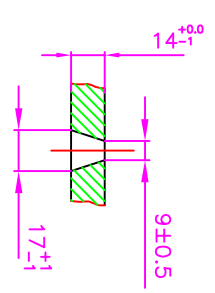
Detail of Holes M=1:1
